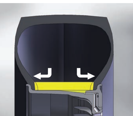
BeadLock effort on tyre wall
