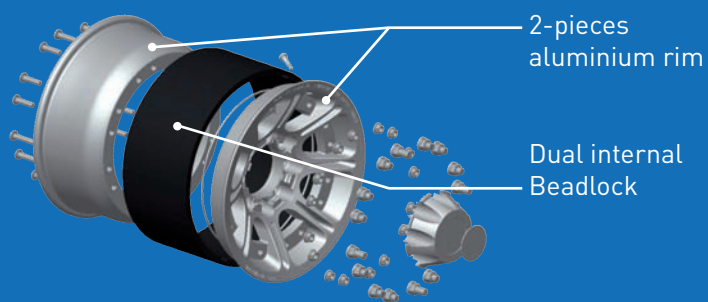
Exploded view Hutchinson wheel assembly
